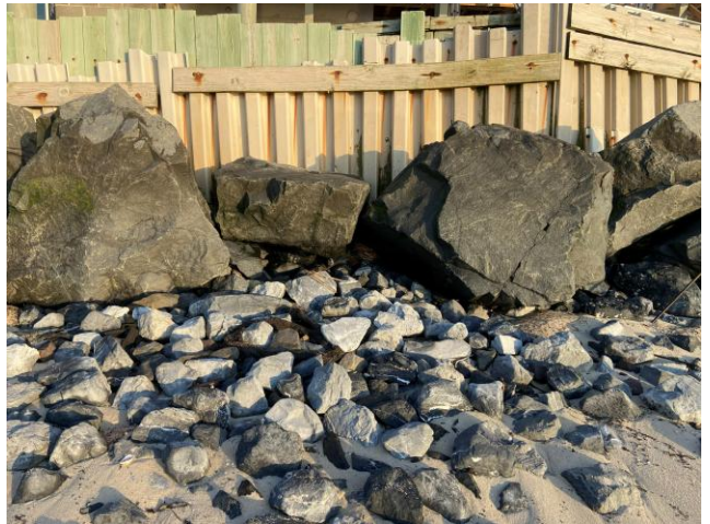
Closeup of bin blocks/riprap surrounding house .
